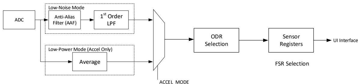
Figure 8. ICM-42607-C Signal Path
