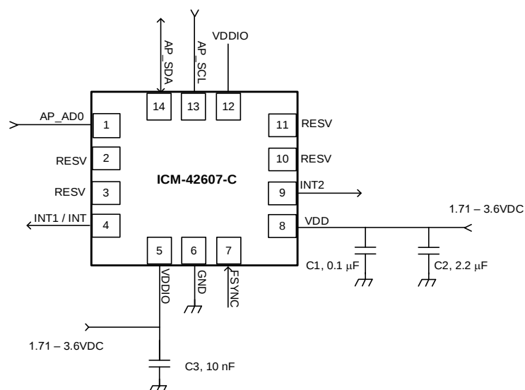
Figure 5. ICM-42607-C Application Schematic (I3C SM / I 2 C Interface to Host)
